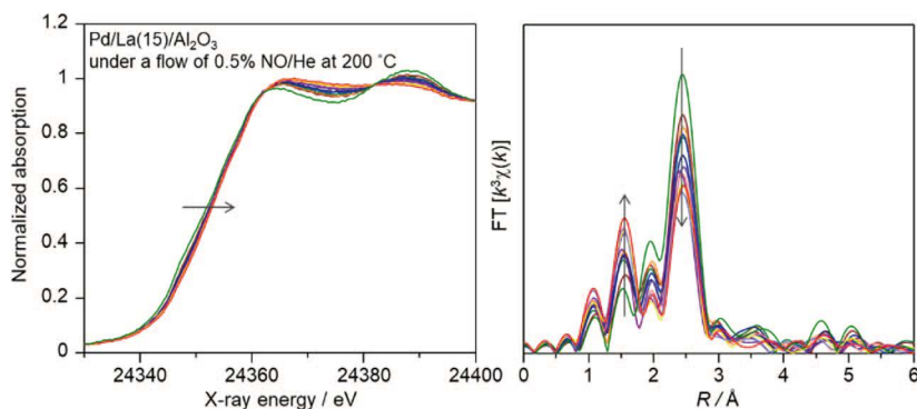
Figure 1. In situ Pd K-edge XANES spectra and EXAFS Fourier transforms of Pd/La(15)/Al 2 O 3 performed under a flow of 0.5% NO/He (800 cm 3 min -1 ) at 200°C after the H 2 reduction at 400°C.
