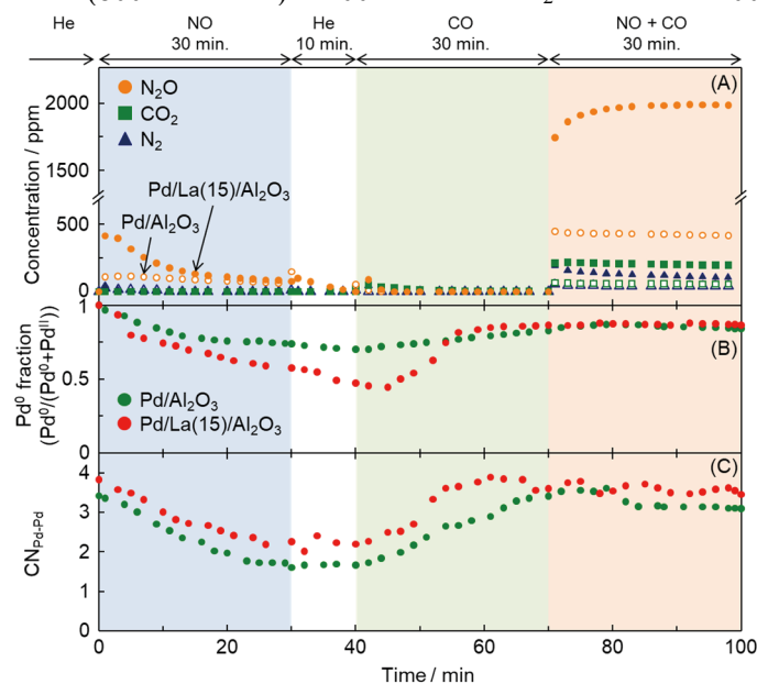
Figure 2. In situ Pd K-edge analysis for Pd/La(15)/Al 2 O 3 and Pd/Al 2 O 3 performed at 200°C. Changes in the fraction of Pd 0 and coordination numbers of the Pd-Pd shell (CN Pd-Pd ) during contact with NO, CO, and NO+CO at 200°C are given with the corresponding changes of the products concentration in the gas phase.
